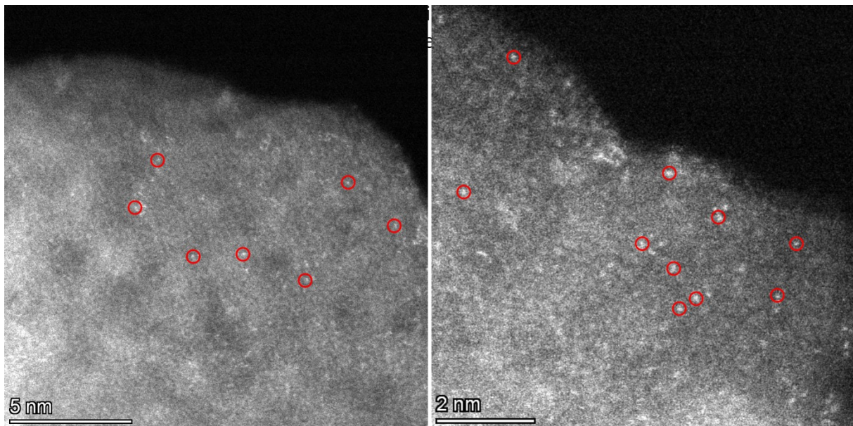
Fig. 1: High-resolution image of the individual copper atoms (marked in red) of the heterogeneous catalyst (Cu-SAC) using a scanning transmission electron microscope (STEM). Fig.: LIKAT
